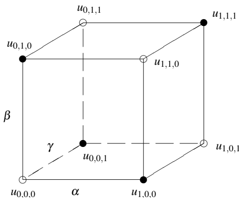
FIGURE 3. Three-dimensional consistency
