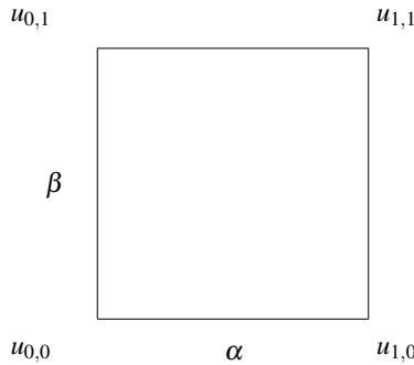
FIGURE 2. A square lattice
